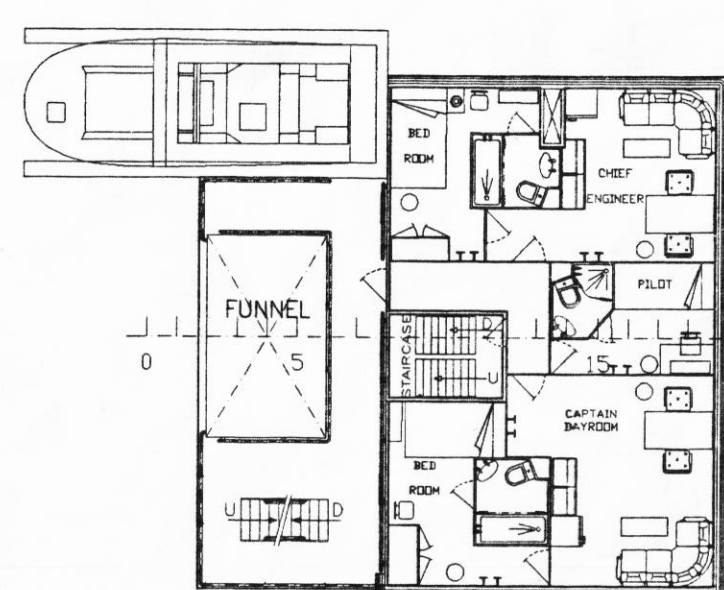
CAPTAINS DECK
