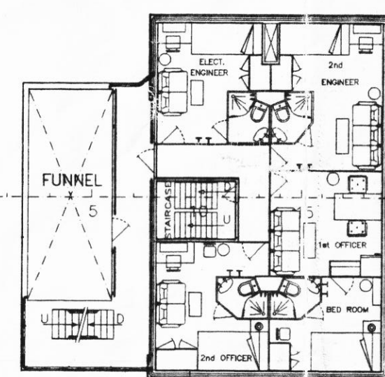
OFFICERS DECK
