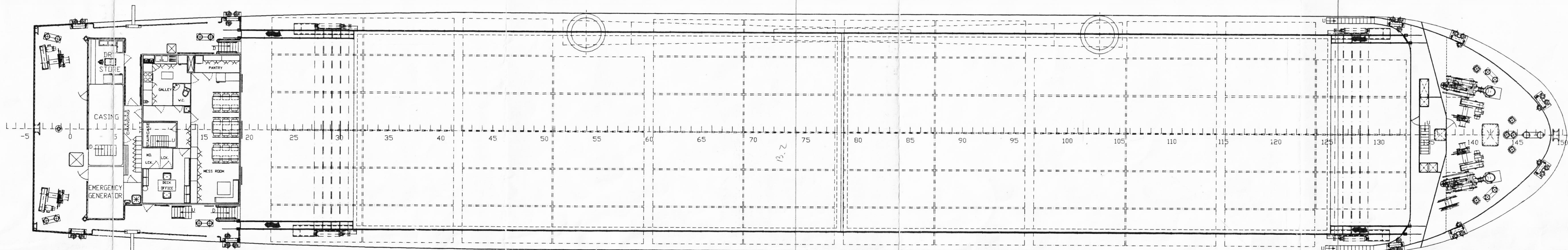
POOP DECK
