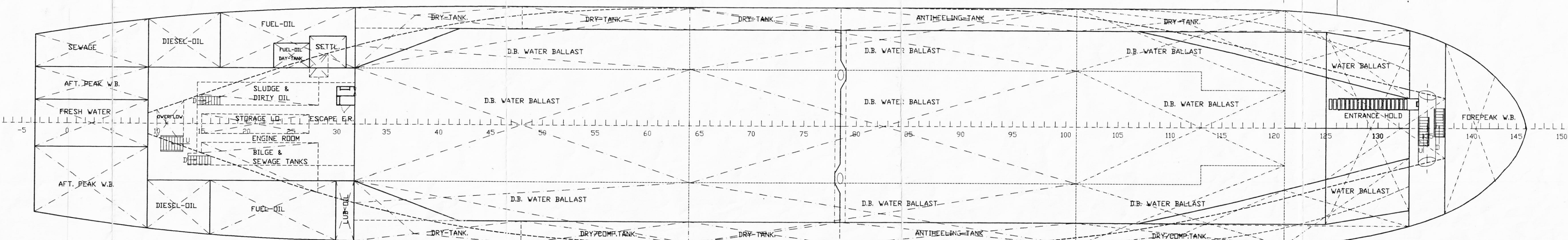
TANKTOP
