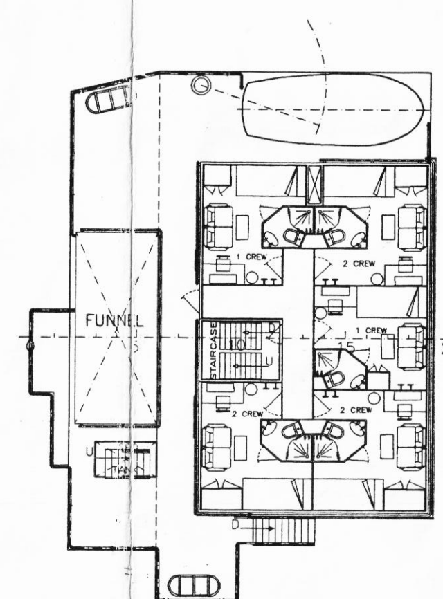
BOAT DECK
